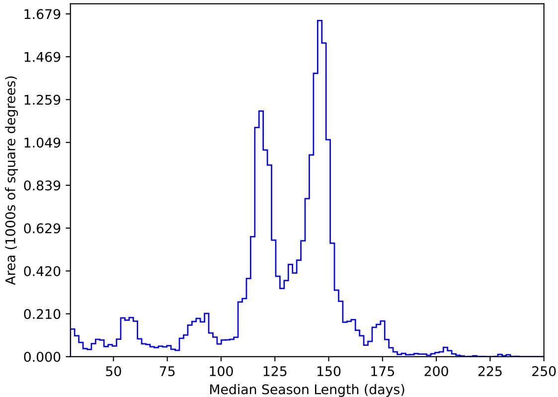
too_elab_r128_d3_ugrizy_v3.4_10yrs All sky y band: Median Season Length
