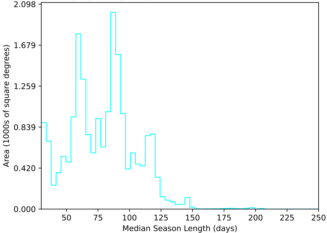
too_elab_r128_d3_ugrizy_v3.4_10yrs All sky u band: Median Season Length
