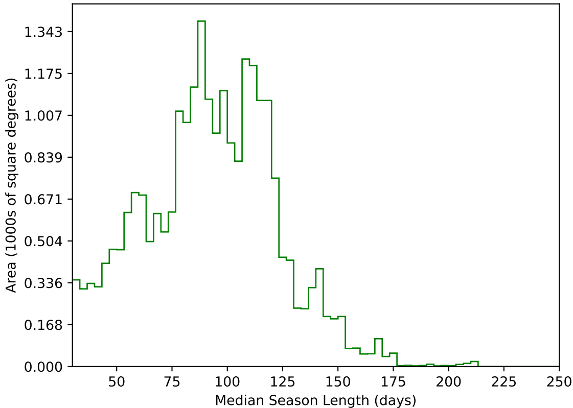
too_elab_r128_d3_ugrizy_v3.4_10yrs All sky g band: Median Season Length
