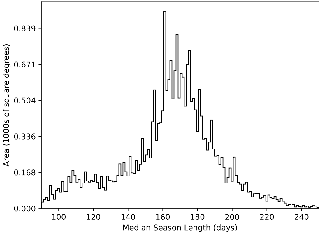
too_elab_r128_d3_ugrizy_v3.4_10yrs All sky all bands: Median Season Length
