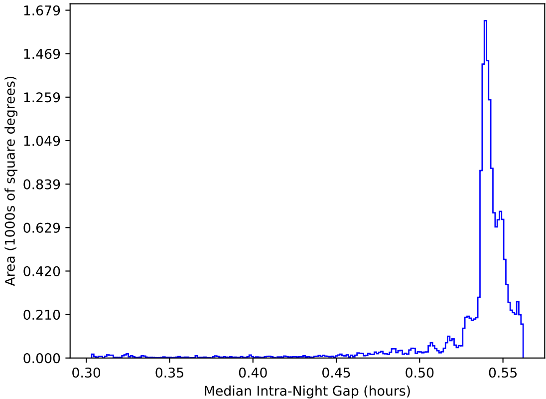
too_elab_r128_d3_ugrizy_v3.4_10yrs WFD: Median Intra-Night Gap
