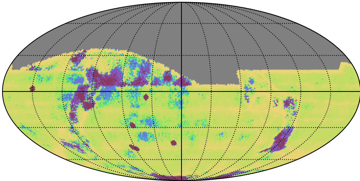
too_elab_r128_d3_ugrizy_v3.4_10yrs All sky: Median Intra-Night Gap
