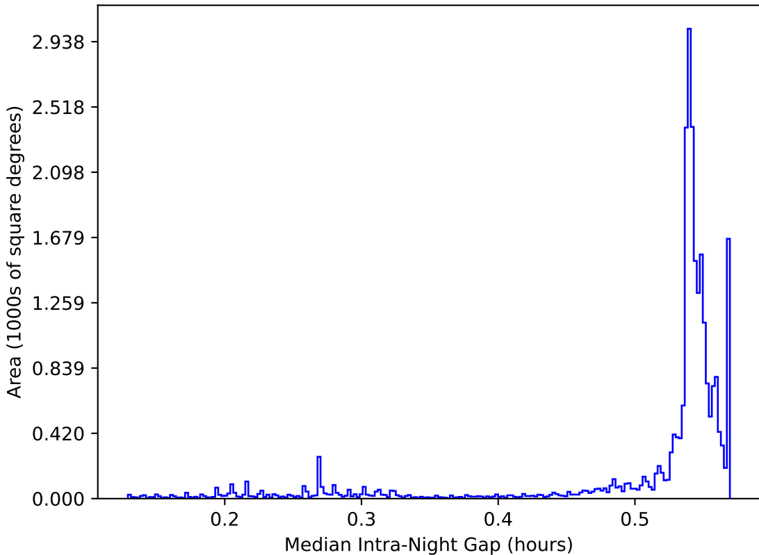
too_elab_r128_d3_ugrizy_v3.4_10yrs All sky: Median Intra-Night Gap
