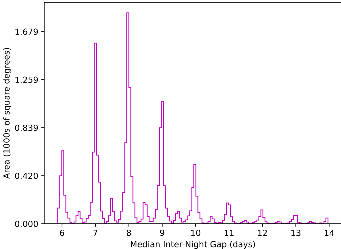
too_elab_r128_d3_ugrizy_v3.4_10yrs WFD z band: Median Inter-Night Gap
