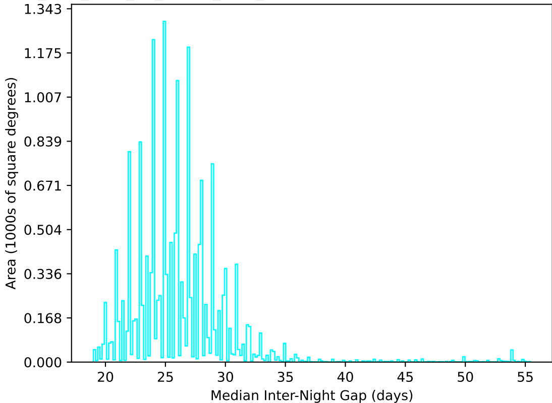
too_elab_r128_d3_ugrizy_v3.4_10yrs WFD u band: Median Inter-Night Gap
