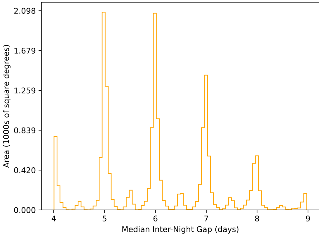
too_elab_r128_d3_ugrizy_v3.4_10yrs WFD r band: Median Inter-Night Gap
