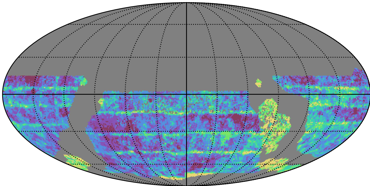
too_elab_r128_d3_ugrizy_v3.4_10yrs WFD i band: Median Inter-Night Gap
