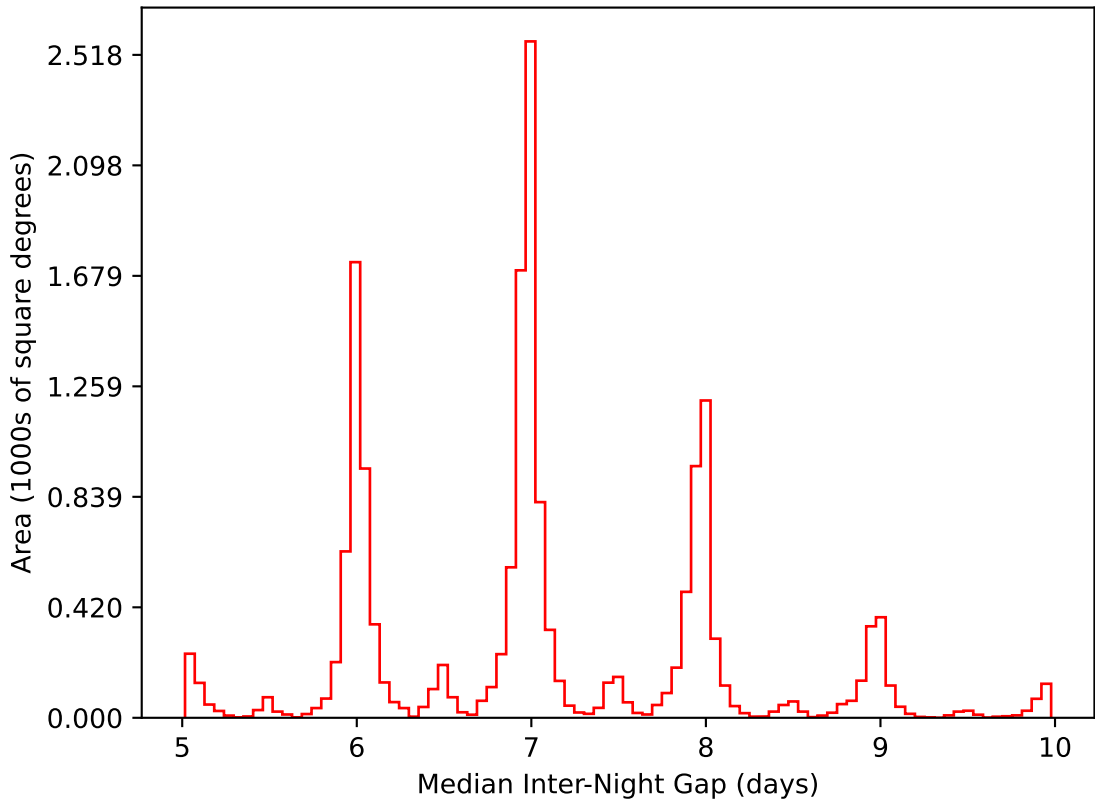
too_elab_r128_d3_ugrizy_v3.4_10yrs WFD i band: Median Inter-Night Gap
