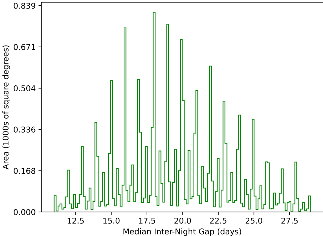
too_elab_r128_d3_ugrizy_v3.4_10yrs WFD g band: Median Inter-Night Gap
