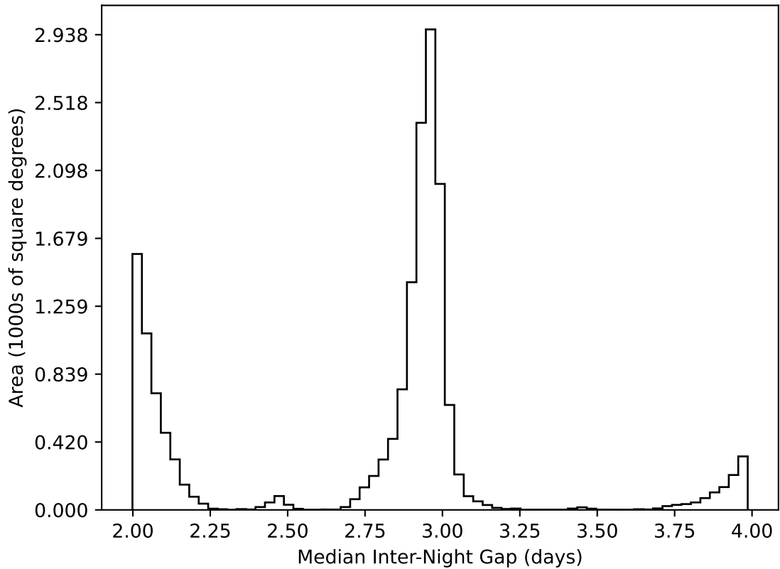
too_elab_r128_d3_ugrizy_v3.4_10yrs WFD all bands: Median Inter-Night Gap
