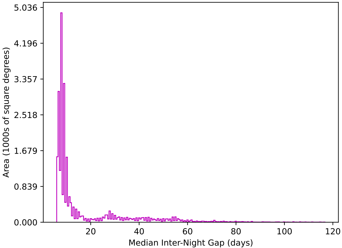
too_elab_r128_d3_ugrizy_v3.4_10yrs All sky z band: Median Inter-Night Gap
