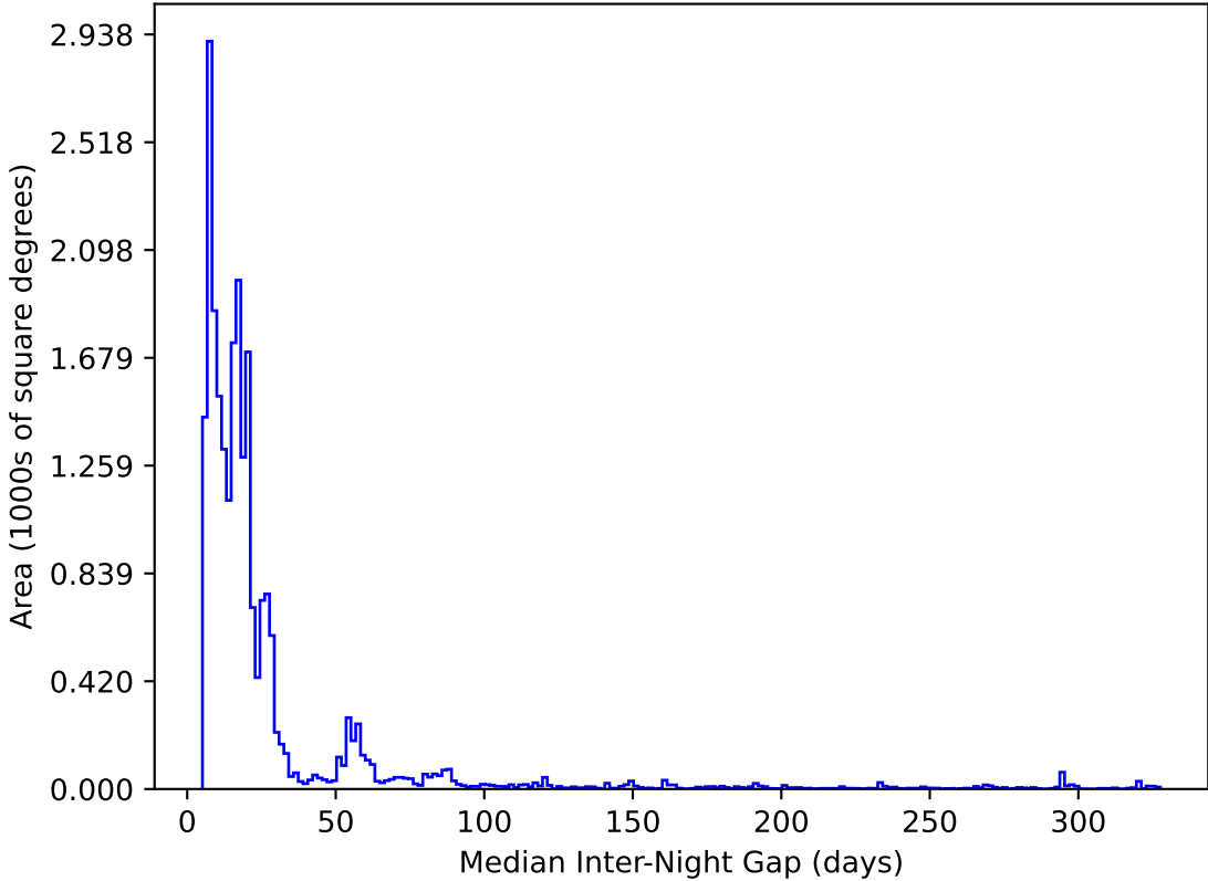
too_elab_r128_d3_ugrizy_v3.4_10yrs All sky y band: Median Inter-Night Gap
