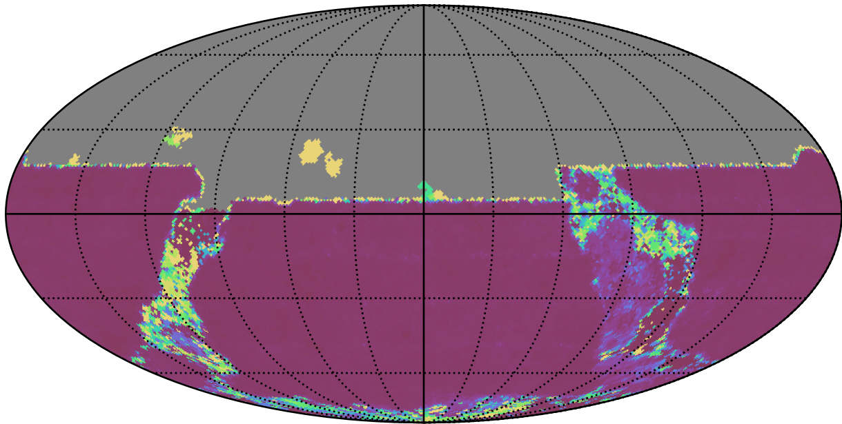
too_elab_r128_d3_ugrizy_v3.4_10yrs All sky u band: Median Inter-Night Gap
