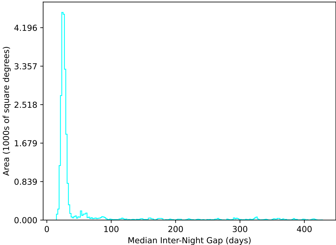
too_elab_r128_d3_ugrizy_v3.4_10yrs All sky u band: Median Inter-Night Gap
