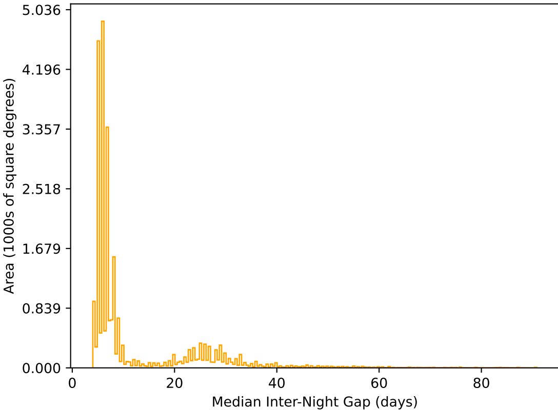
too_elab_r128_d3_ugrizy_v3.4_10yrs All sky r band: Median Inter-Night Gap
