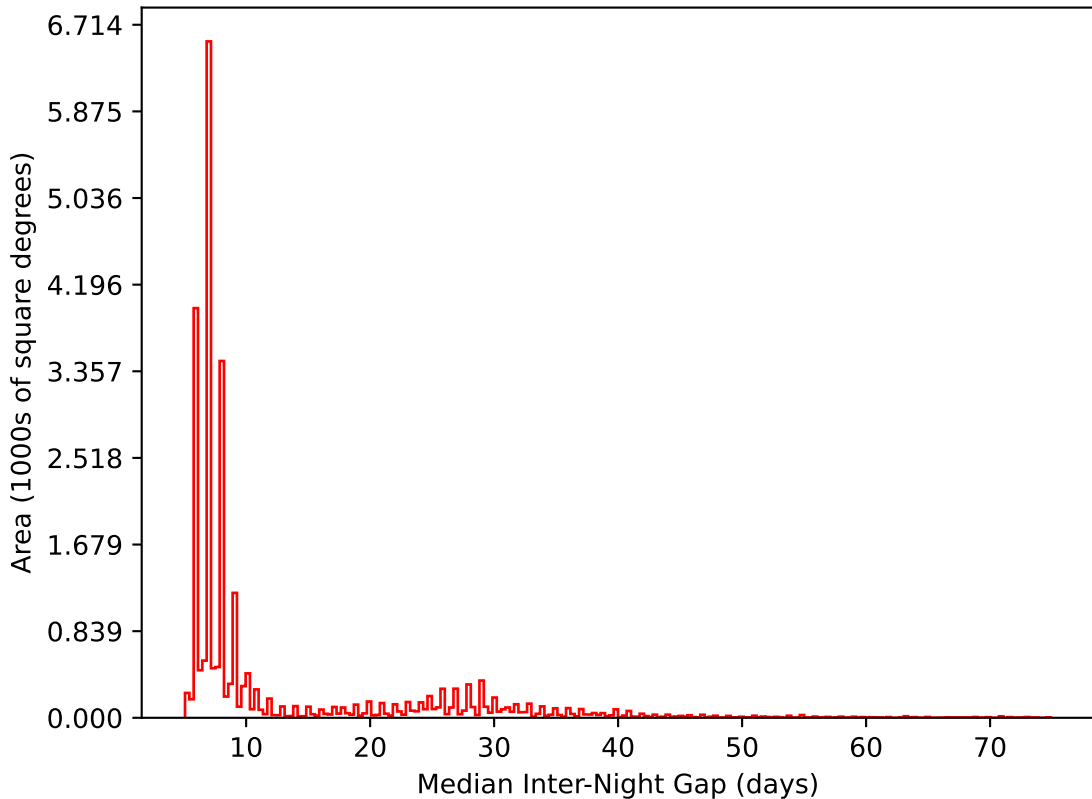
too_elab_r128_d3_ugrizy_v3.4_10yrs All sky i band: Median Inter-Night Gap
