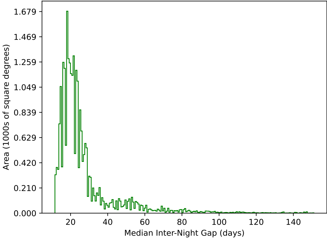
too_elab_r128_d3_ugrizy_v3.4_10yrs All sky g band: Median Inter-Night Gap
