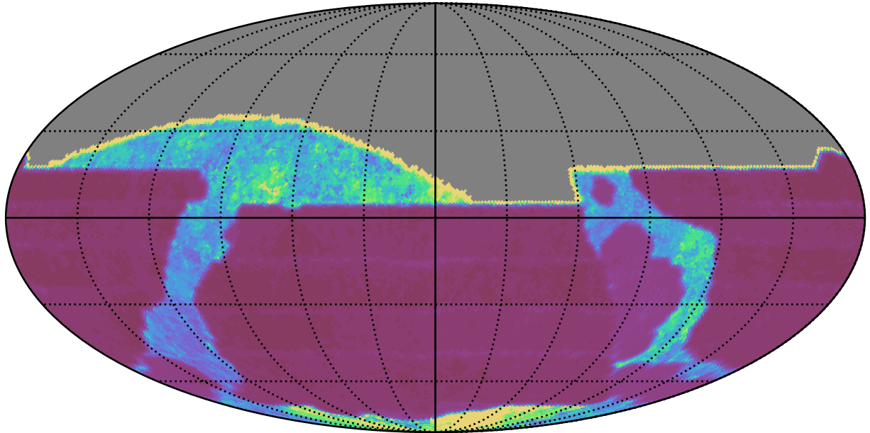
too_elab_r128_d3_ugrizy_v3.4_10yrs All sky all bands: Median Inter-Night Gap
