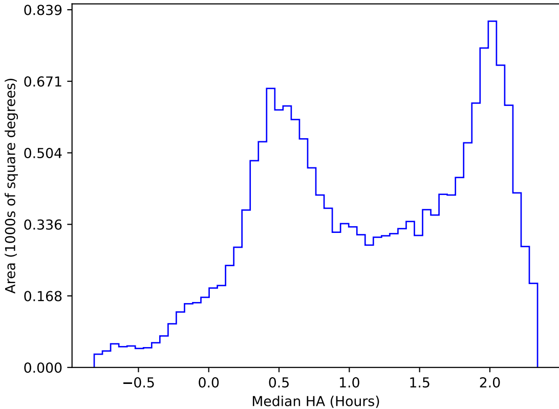
too_elab_r128_d3_ugrizy_v3.4_10yrs WFD z band: Median HA
