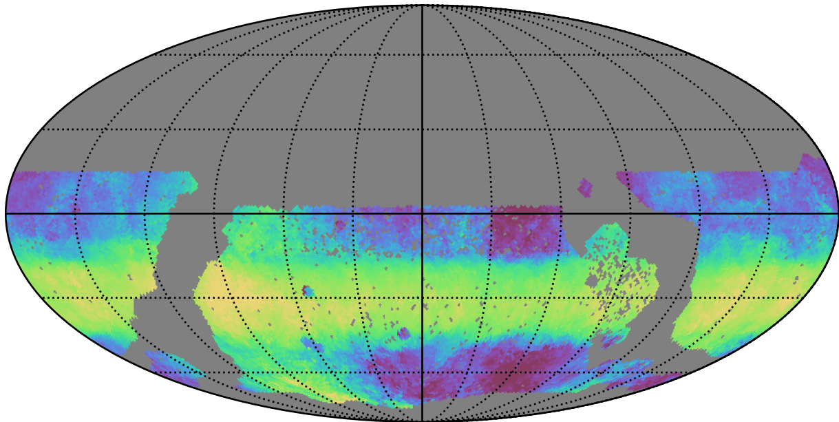
too_elab_r128_d3_ugrizy_v3.4_10yrs WFD y band: Median HA
