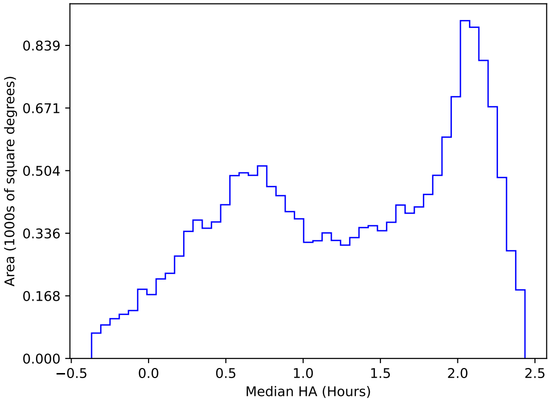
too_elab_r128_d3_ugrizy_v3.4_10yrs WFD y band: Median HA
