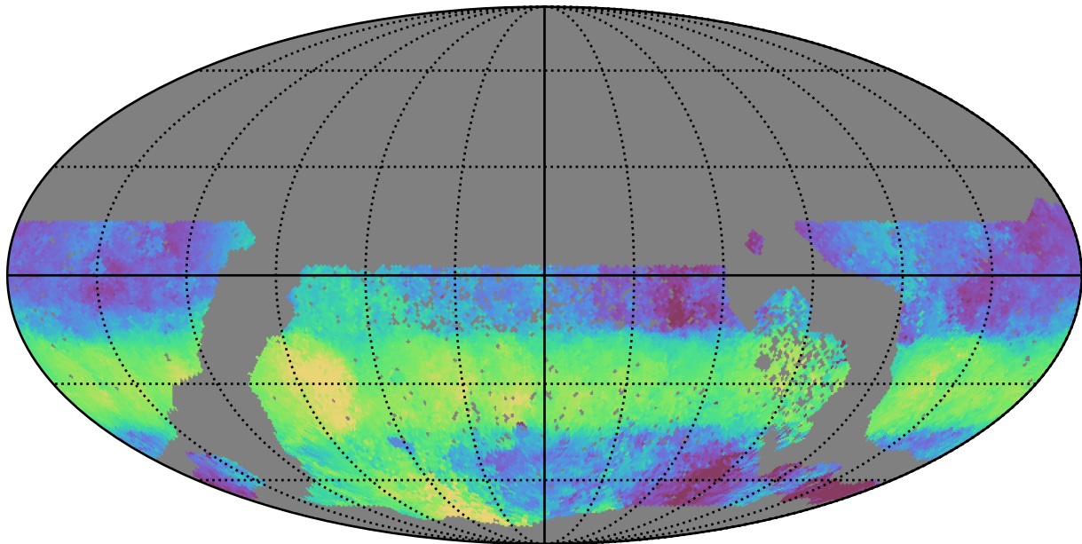
too_elab_r128_d3_ugrizy_v3.4_10yrs WFD u band: Median HA
