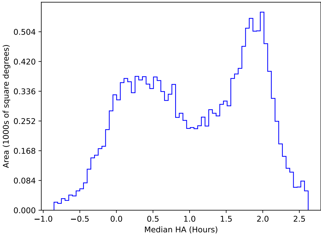
too_elab_r128_d3_ugrizy_v3.4_10yrs WFD u band: Median HA
