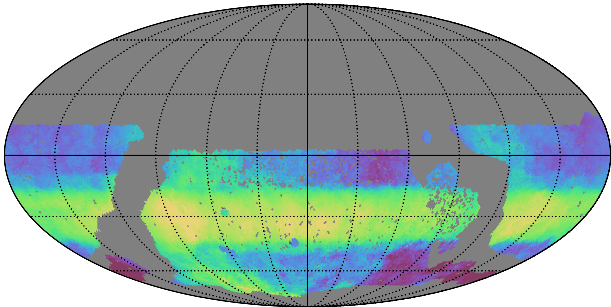
too_elab_r128_d3_ugrizy_v3.4_10yrs WFD r band: Median HA
