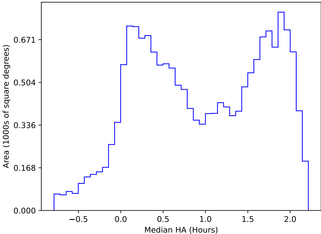
too_elab_r128_d3_ugrizy_v3.4_10yrs WFD r band: Median HA
