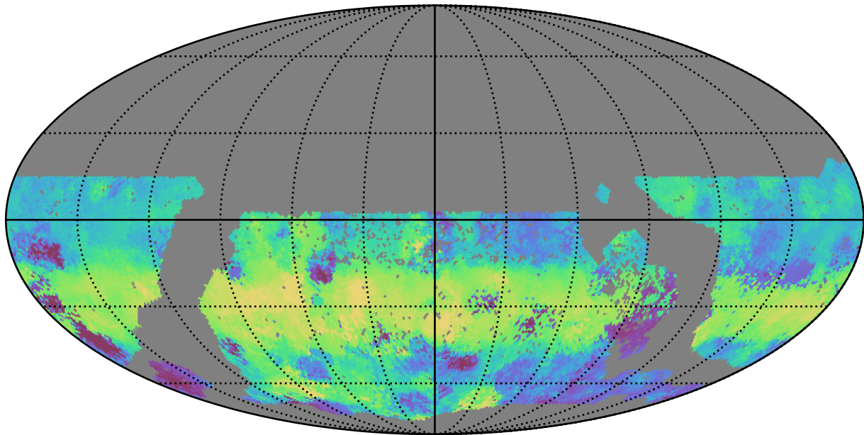
too_elab_r128_d3_ugrizy_v3.4_10yrs WFD g band: Median HA
