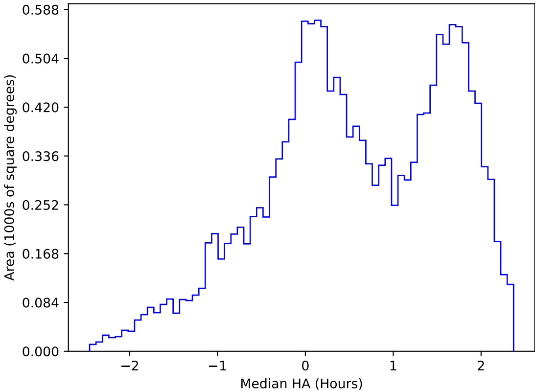
too_elab_r128_d3_ugrizy_v3.4_10yrs WFD g band: Median HA
