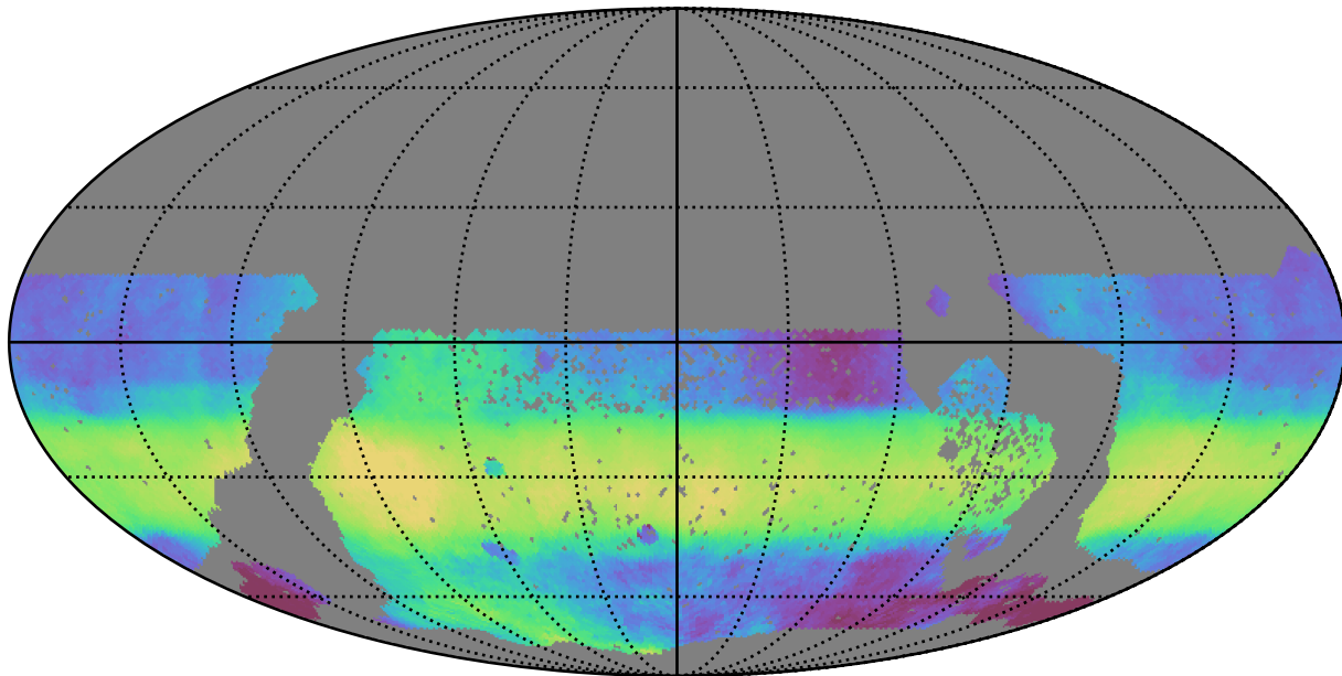
too_elab_r128_d3_ugrizy_v3.4_10yrs WFD all bands: Median HA
