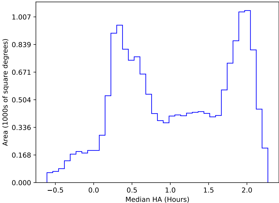
too_elab_r128_d3_ugrizy_v3.4_10yrs WFD all bands: Median HA
