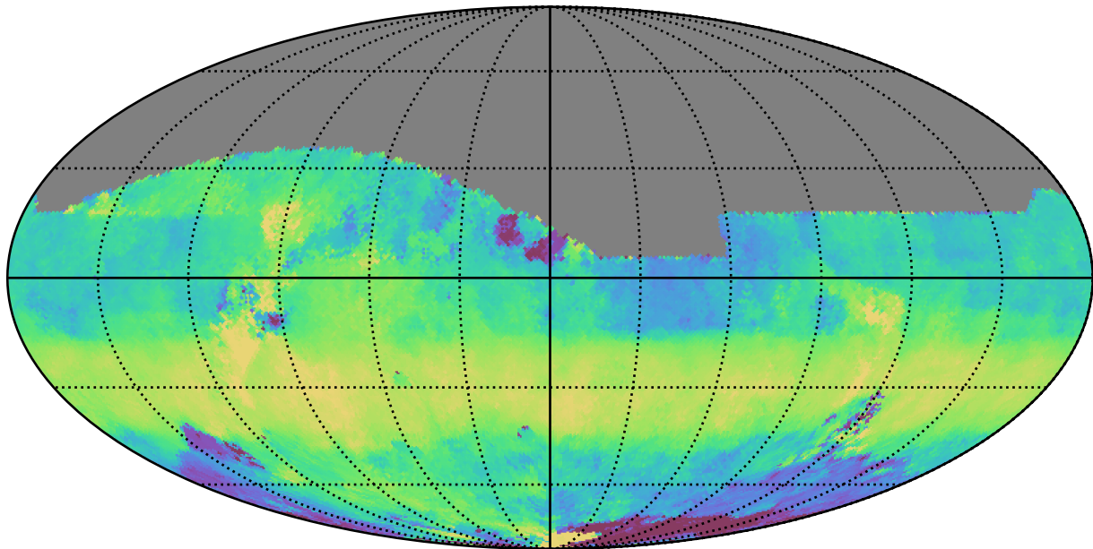
too_elab_r128_d3_ugrizy_v3.4_10yrs All sky z band: Median HA
