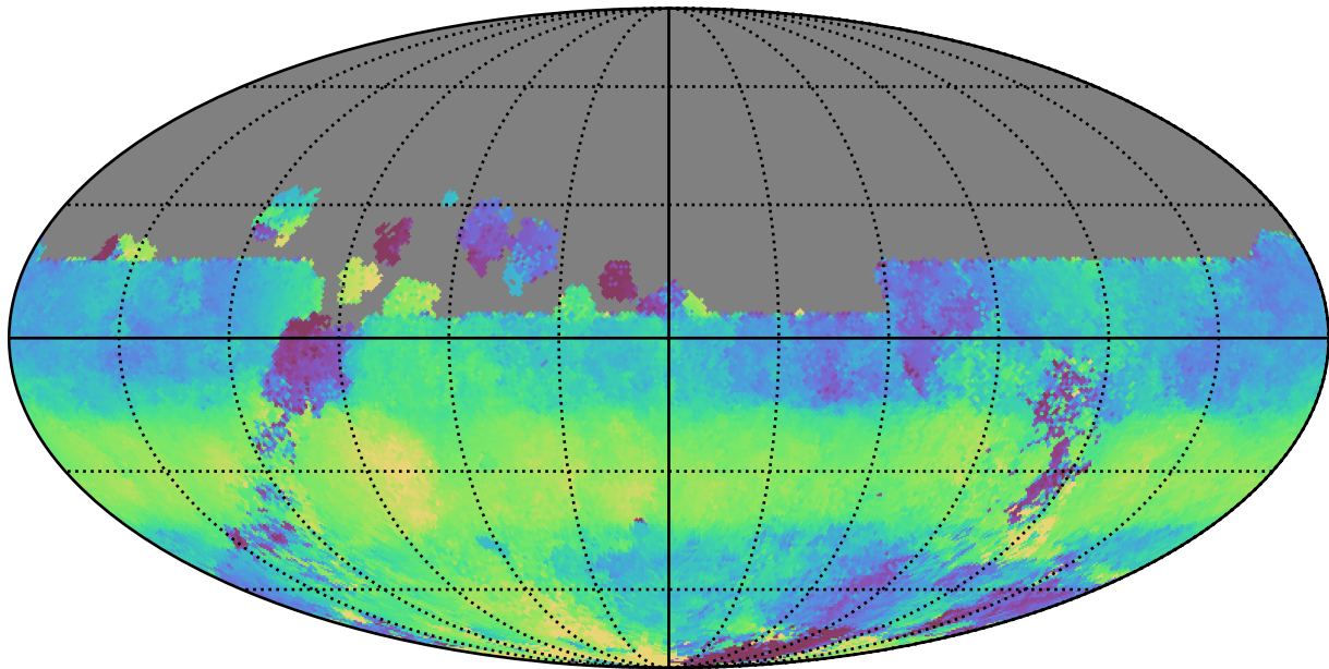
too_elab_r128_d3_ugrizy_v3.4_10yrs All sky u band: Median HA
