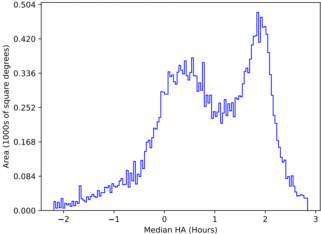
too_elab_r128_d3_ugrizy_v3.4_10yrs All sky u band: Median HA
