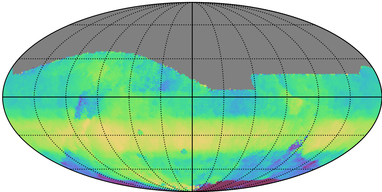
too_elab_r128_d3_ugrizy_v3.4_10yrs All sky r band: Median HA
