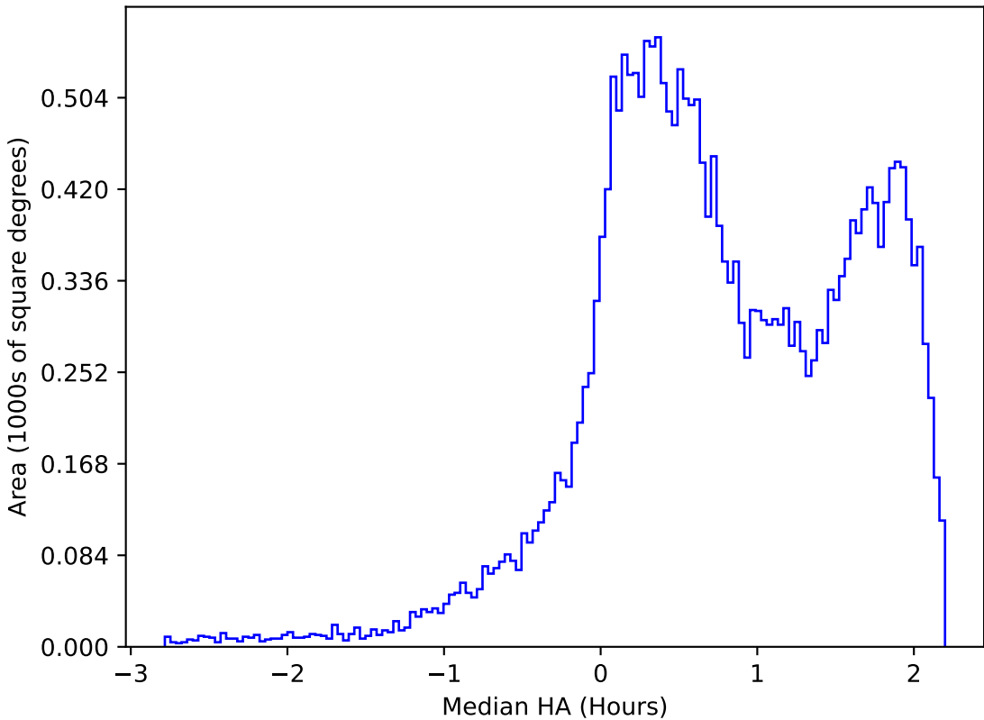
too_elab_r128_d3_ugrizy_v3.4_10yrs All sky r band: Median HA
