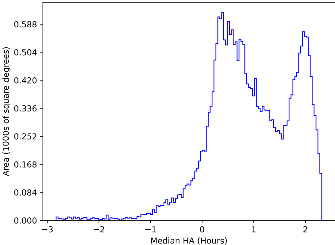
too_elab_r128_d3_ugrizy_v3.4_10yrs All sky i band: Median HA
