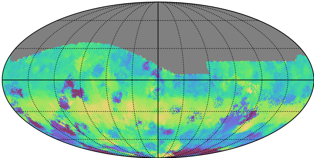
too_elab_r128_d3_ugrizy_v3.4_10yrs All sky g band: Median HA
