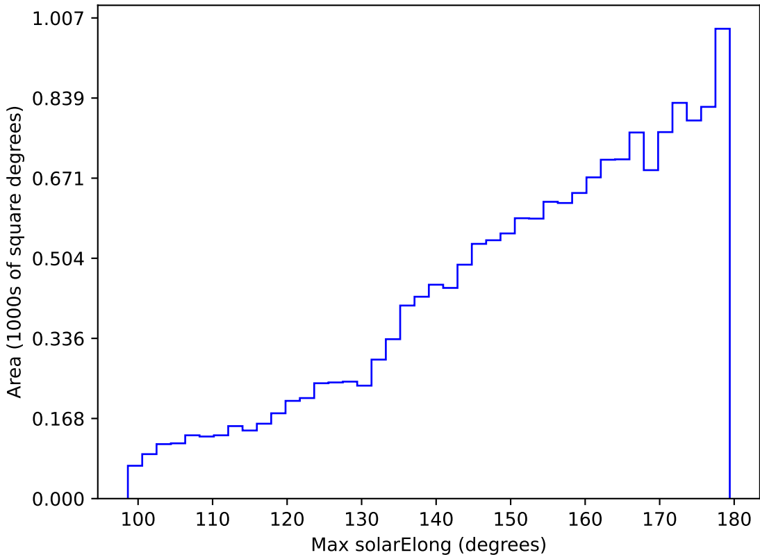
too_elab_r128_d3_ugrizy_v3.4_10yrs WFD z band: Max solarElong
