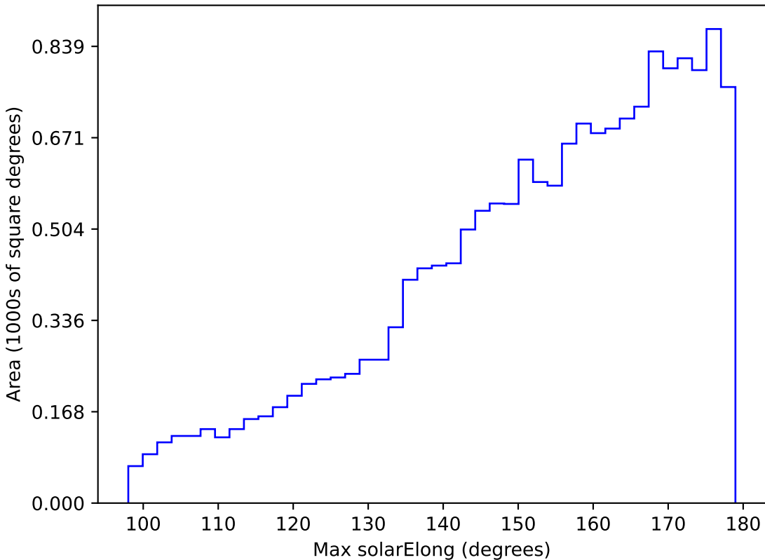
too_elab_r128_d3_ugrizy_v3.4_10yrs WFD u band: Max solarElong
