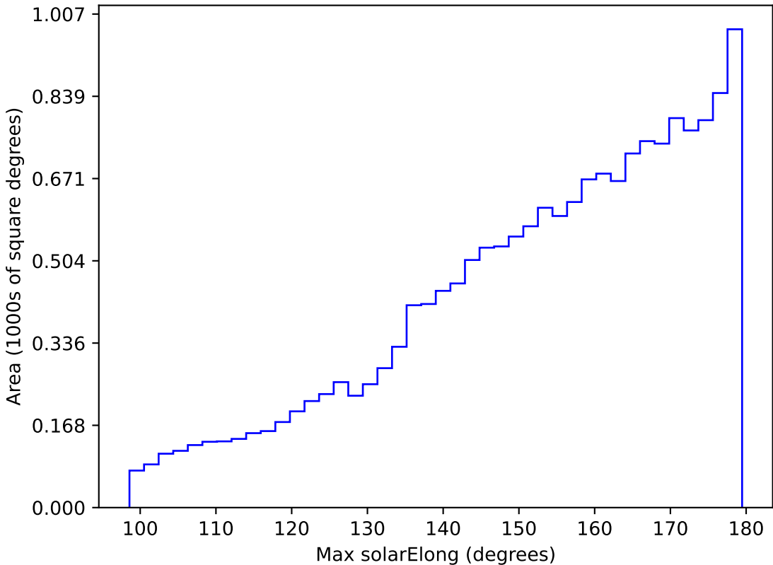
too_elab_r128_d3_ugrizy_v3.4_10yrs WFD r band: Max solarElong
