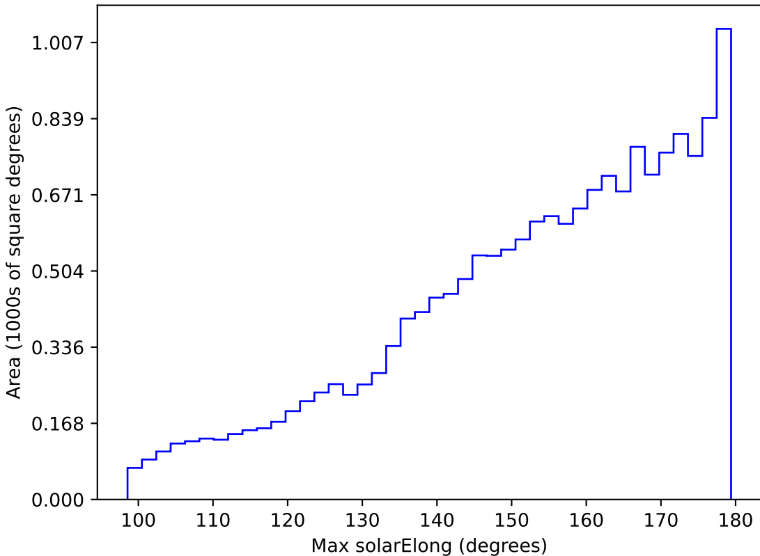
too_elab_r128_d3_ugrizy_v3.4_10yrs WFD i band: Max solarElong
