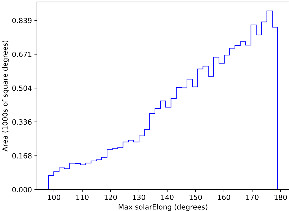
too_elab_r128_d3_ugrizy_v3.4_10yrs WFD g band: Max solarElong
