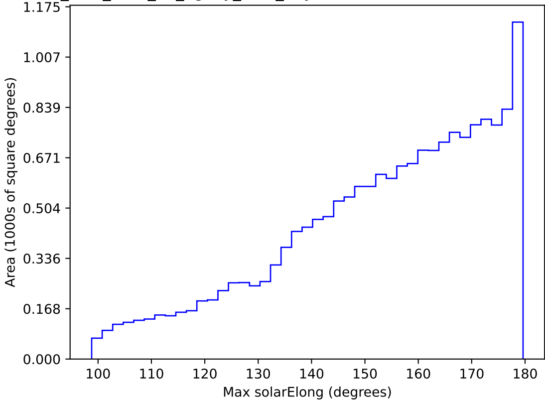
too_elab_r128_d3_ugrizy_v3.4_10yrs WFD all bands: Max solarElong
