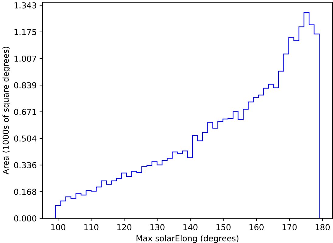
too_elab_r128_d3_ugrizy_v3.4_10yrs All sky g band: Max solarElong
