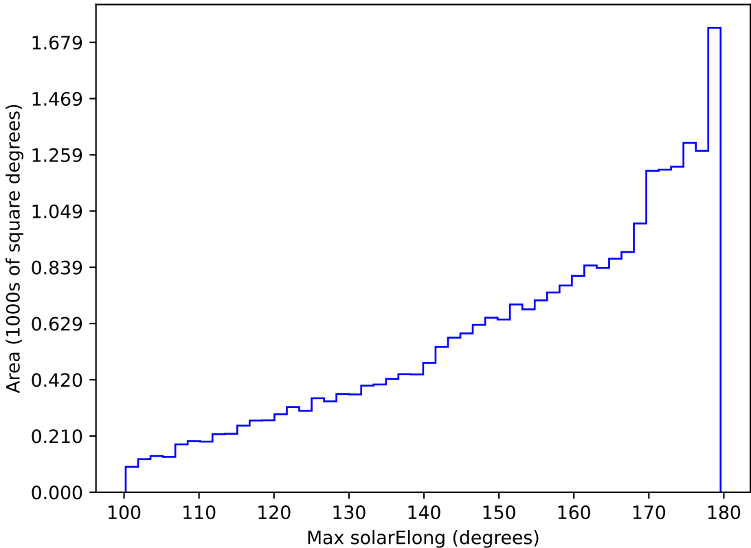
too_elab_r128_d3_ugrizy_v3.4_10yrs All sky all bands: Max solarElong
