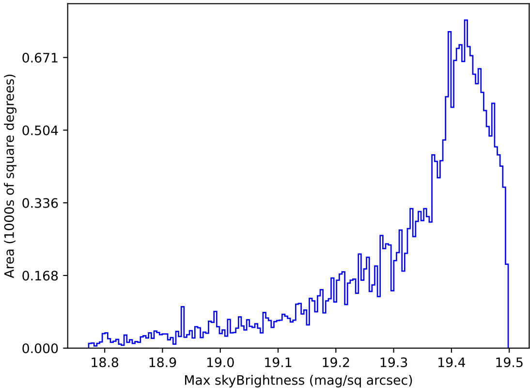
too_elab_r128_d3_ugrizy_v3.4_10yrs Yr 1 z band: Max skyBrightness
