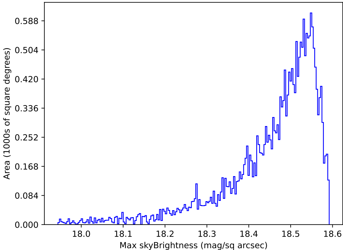
too_elab_r128_d3_ugrizy_v3.4_10yrs Yr 1 y band: Max skyBrightness
